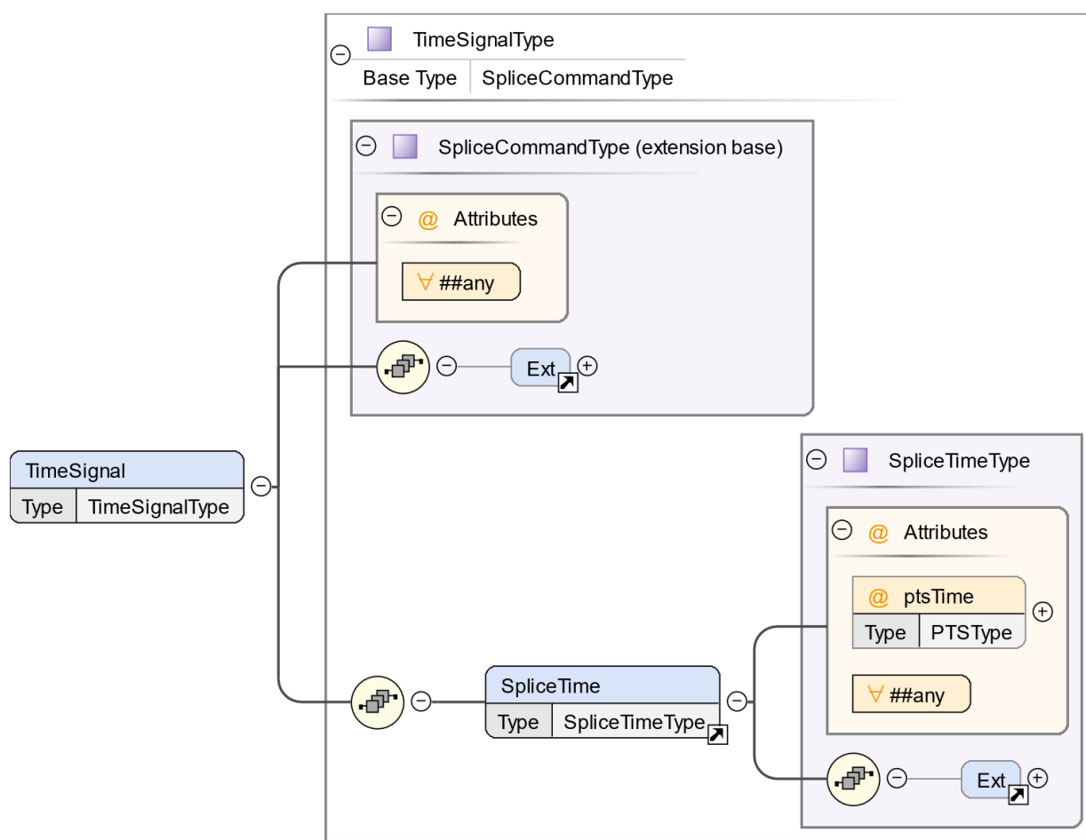
Figure 11 - TimeSignal
