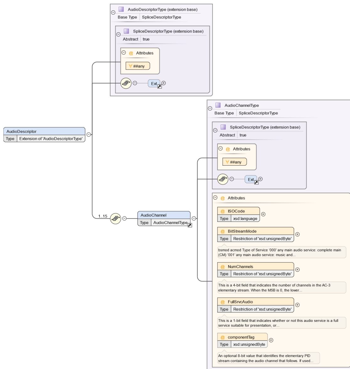
Figure 23 – AudioDescriptor
