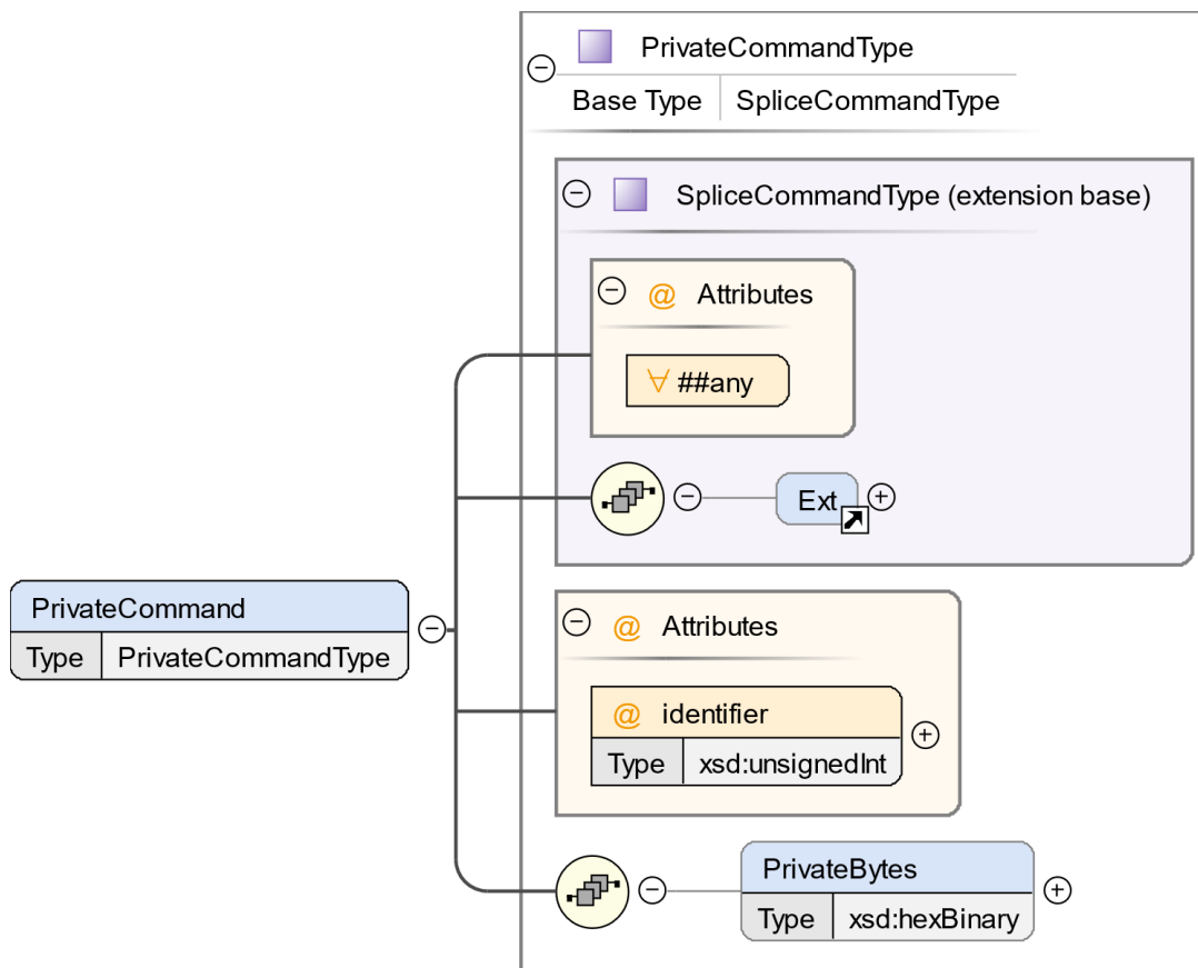
Figure 13 - PrivateCommand
