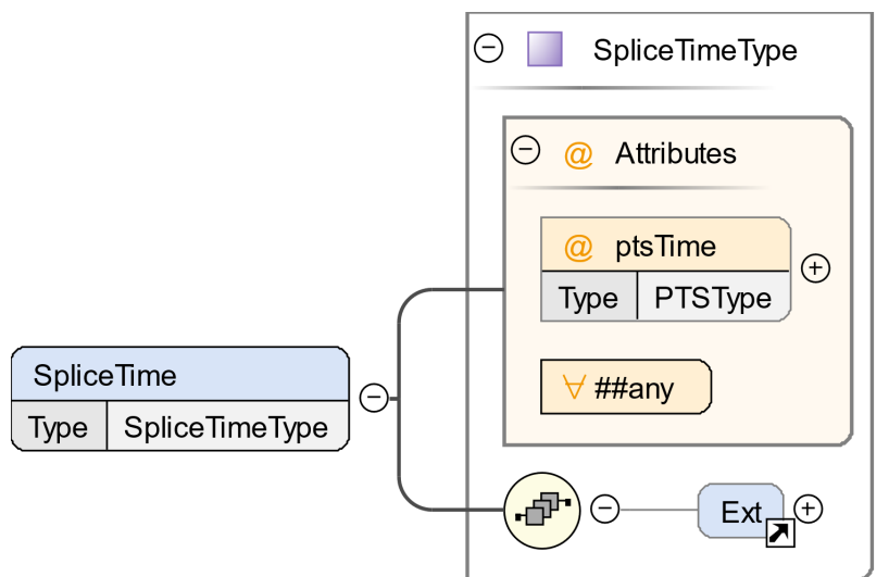
Figure 14 - SpliceTime
