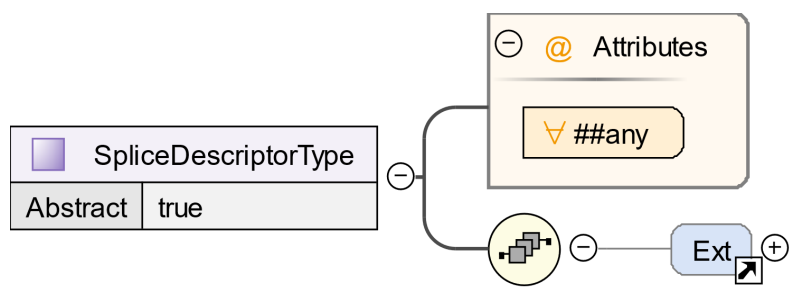
Figure 16 - SpliceDescriptorType
