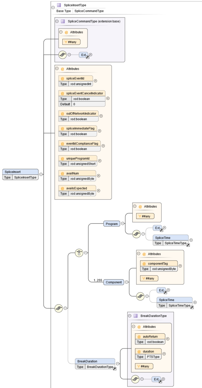
Figure 10 - SpliceInsert
