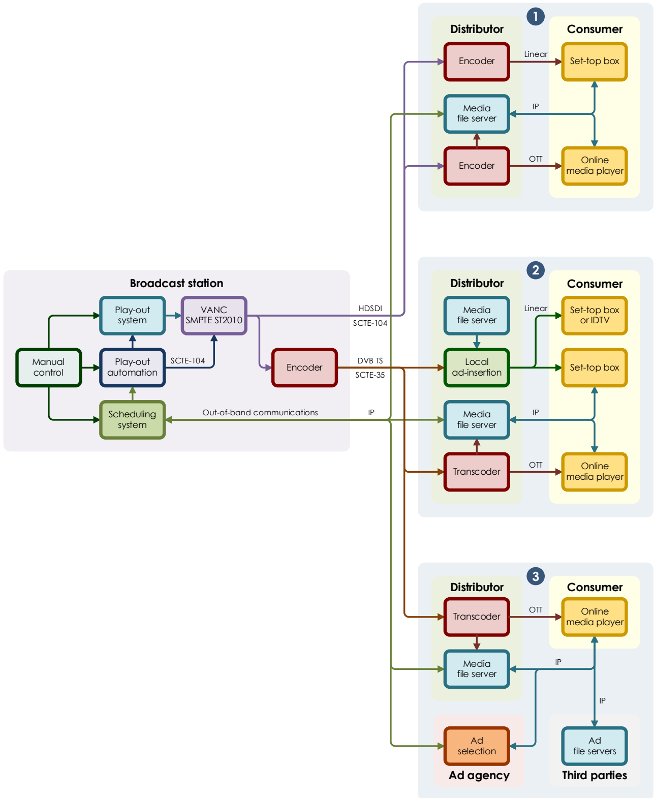
Figure 1 – SCTE 104/35 signal flow examples
